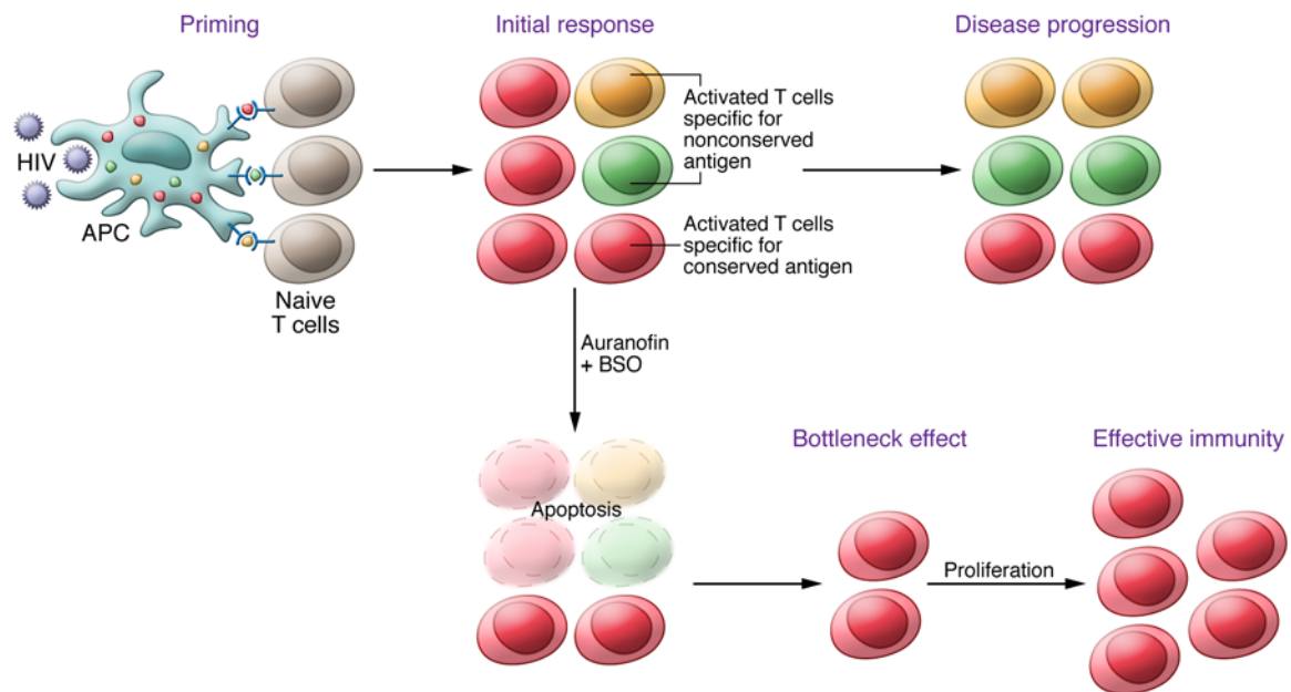
Figure 3. Hypothesized bottleneck mechanism for the enhancement of cell-mediated immunity following inhibition of the Trx and GSH systems. A professional APC (DC) can phagocytize a foreign pathogen (HIV), degrade it into peptidic antigens, and present these antigens to naive lymphocytes. Because of high mutation rates, HIV antigens are characterized by high variability, with the exception of highly conserved, essential proteins, which are consequently well represented in a typical viral population. Following antigen presentation, the lymphocyte becomes activated and primed toward a specific antigen. During the progression of HIV infection (upper panel), the lymphocyte clones specific for conserved antigens (red halo in the figure) are reduced in frequency due to the accumulation of “nonfunctional clones” directed against increasingly mutated antigens (green and gold halos). When Trx and GSH systems are inhibited, lymphocyte activation is impaired, and the majority of activated lymphocyte clones undergo stochastic apoptosis. The more frequently represented clones have a selective advantage in survival as a result of their numbers. This leads to a bottleneck effect that can favor repopulation by those lymphocytes primed against the most frequently represented (conserved) antigens.
