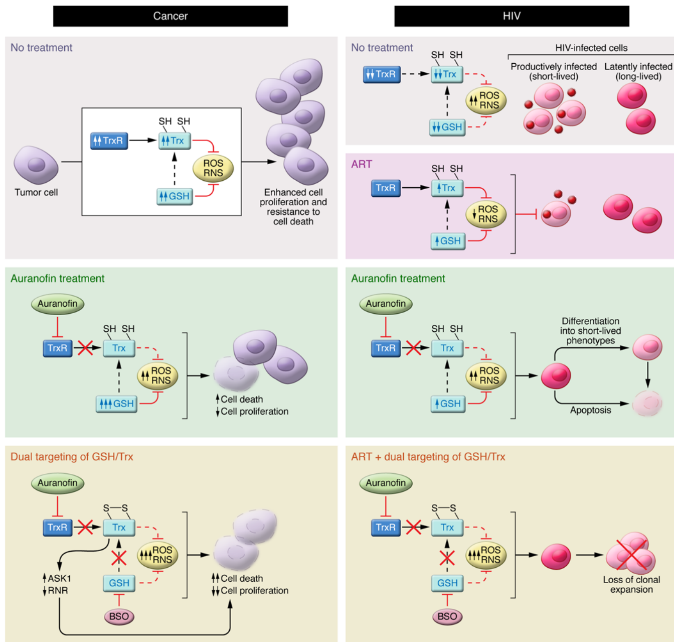
Figure 2. Model of the anticancer and anti-HIV effects of targeting the Trx and GSH systems. Left: Many cancer cells generate large amounts of ROS and RNS but also have elevated antioxidant defenses, largely through upregulation of the Trx and GSH systems. Inhibition of TrxR by auranofin can lead to elevated ROS and RNS levels, apoptosis, and decreased cell proliferation. However, when TrxR is inhibited, the GSH redox system often becomes upregulated, eliminating ROS and RNS and acting as a backup system to reduce Trx. Exposure of cancer cells to auranofin and BSO disables both Trx and GSH systems, severely compromising antioxidant capacity and leading to marked elevation of ROS and SNOs, which suppress cell proliferation and promote cell death. Cell death is in part mediated by inhibition of ribonucleotide reductase (RNR) and through activation of the proapoptotic kinase ASK1. Right: HIV-infected cells are characterized by elevated levels of ROS, coupled with decreased intracellular levels of antioxidant defenses (Trx, TrxR, and GSH). ART blocks HIV replication and partially counteracts the effects of oxidative stress, but is unable to target the latently infected cells. Inhibition of TrxR by auranofin increases oxidative (and potentially nitrosative) stress and apoptosis. TrxR inhibition also leads to a prodifferentiation effect on the latently HIV-infected cells, driving them toward short-lived phenotypes (i.e., effector memory) and, ultimately, decreasing the viral reservoir. Auranofin and BSO impair lymphocyte activation and increase HIV-infected cell death. ROS variations are documented, whereas RNS variations are predicted. Arrows beside the names of the molecules indicate the variation over time. SH, thiol.
