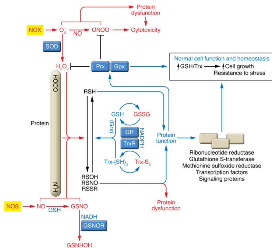
Figure 1. Role of the Trx and GSH systems in cellular nitroso-redox homeostasis and signaling.
