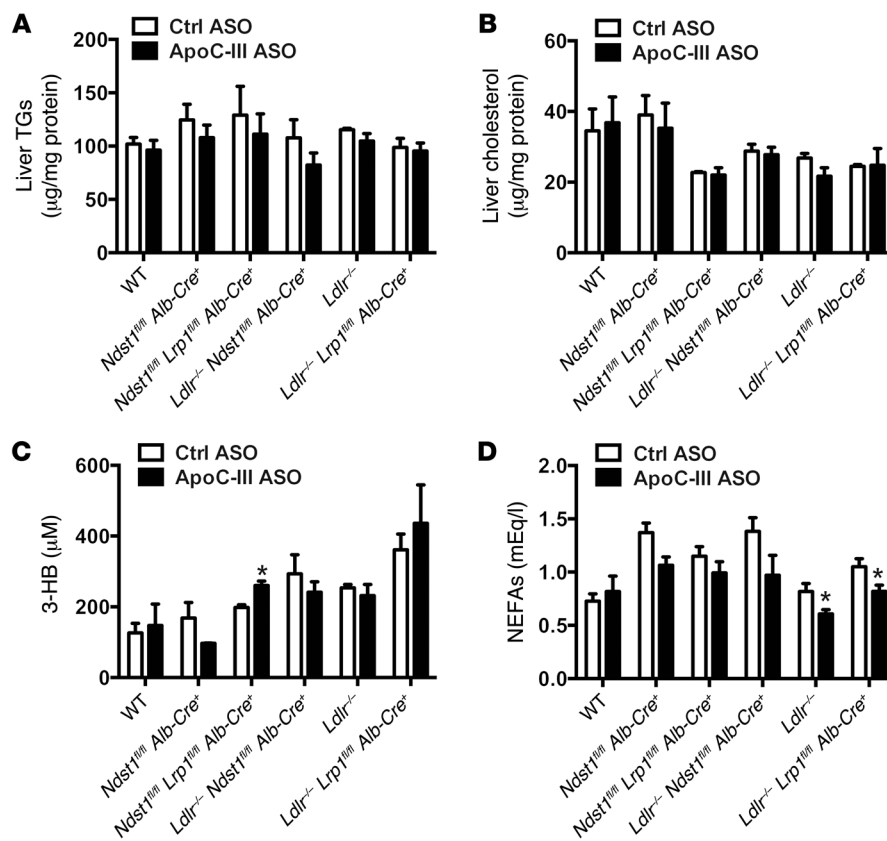
Figure 3. ApoC-III ASO does not induce liver steatosis or production of ketone bodies. (A) Liver TG levels in mutant mice treated for 4 weeks with control or ApoC-III ASO ( n = 3-5 /group). (B) Liver cholesterol levels in mutant mice treated for 4 weeks with control or ApoC-III ASO ( n = 3-5 /group). (C) Fasting plasma levels of 3-hydroxybutyrate (3-HB) in mutant mice treated for 4 weeks with control or ApoC-III ASO ( n = 3-9 /group). (D) Fasting plasma NEFA levels in mutant mice treated for 4 weeks with control or ApoC-III ASO ( n = 3-9 /group). Values represent the mean \pm SEM. * P < 0.05 compared with control ASO-treated mice. ANOVA with Bonferroni's post-hoc test.
